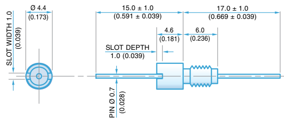
M3.5 x 0.5 - 6g Thread 4.4mm Round Head
