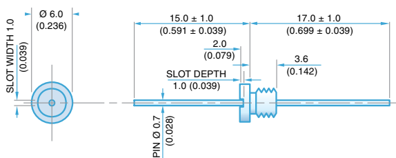
Low Profile M5 x 0.8 - 6g Thread 6.0mm Round Head
